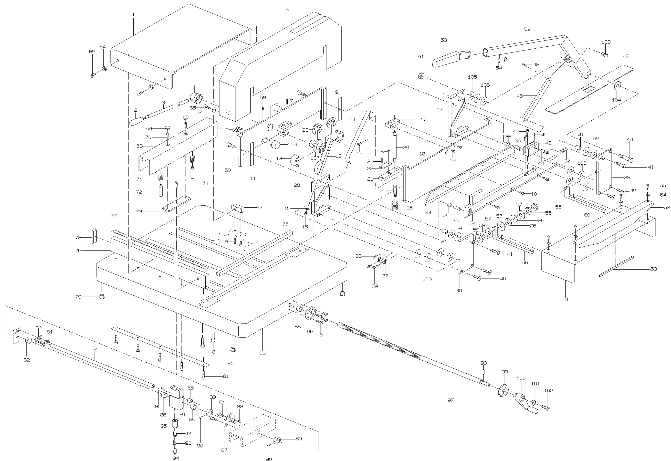
Abbildung 1 Stapelschneider 848 Illustration 1 Ream cutter 848 Illustration 1 Massicot 848
