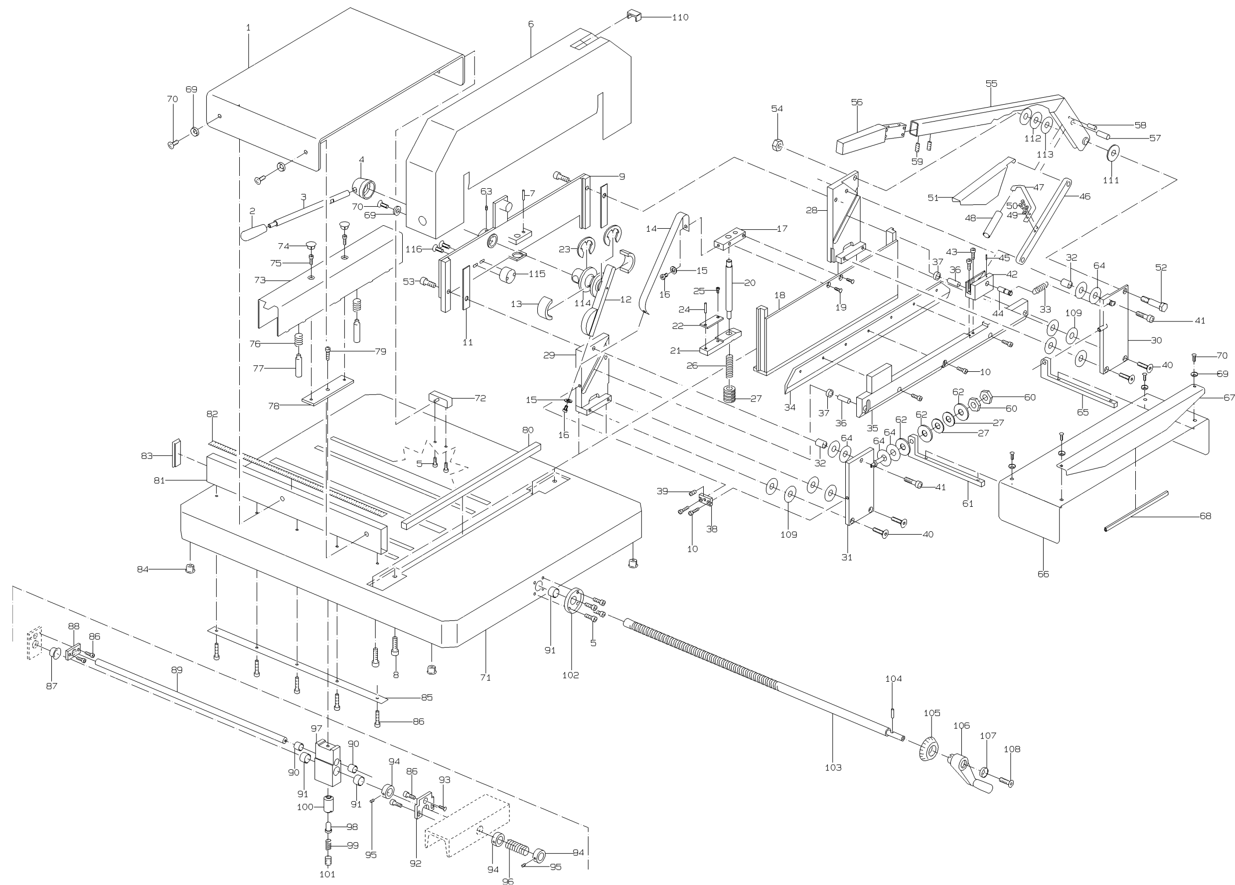
Abbildung 1 Stapelschneider 846 Illustration 1 Ream cutter 846 Illustration 1 Massicot 846
